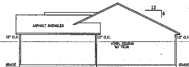
RIGHT ELEVATION 1/16" = 1'-0"
