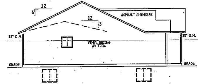
LEFT ELEVATION 1/16" = 1'-0"
