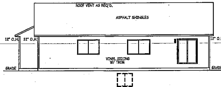
REAR ELEVATION 1/16" = 1'-0"
