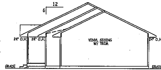
RIGHT ELEVATION 1/16" = 1'-0"
