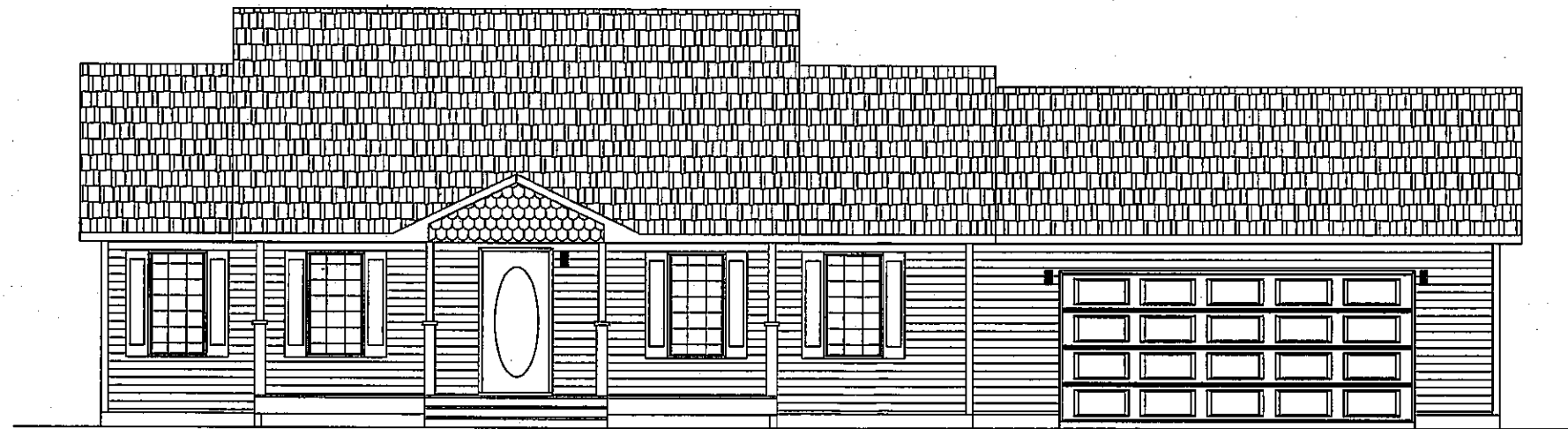
FRONT ELEVATION 1/8" = 1'-0"
