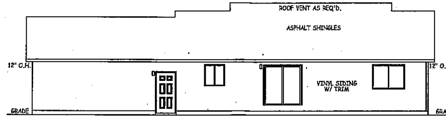
REAR ELEVATION 1/16" = 1'-0"
